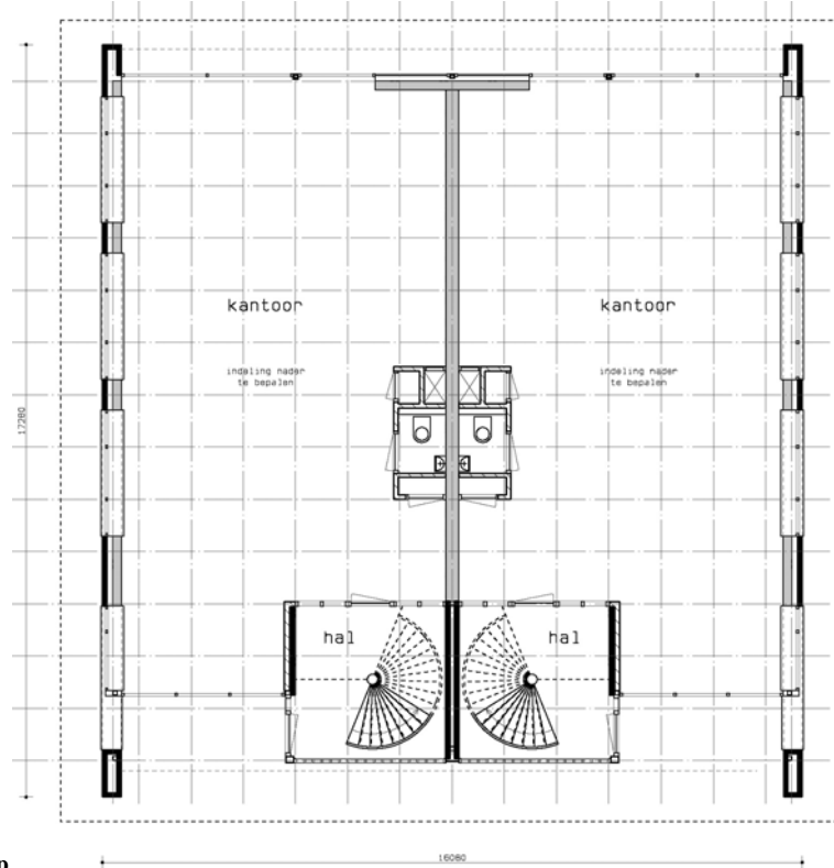
Begane grond 2/1 kap
