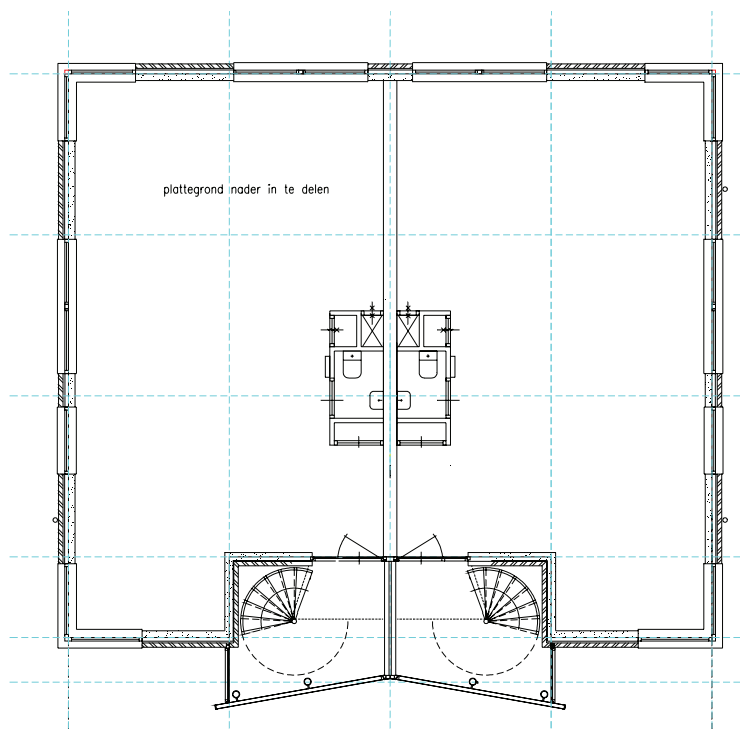
2/1 KAP VERDIEPING
